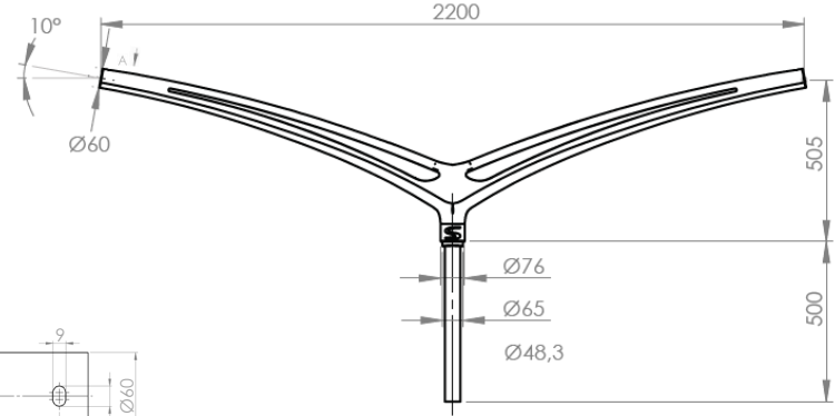
ELAYA TOP DOUBLE 1100 / Pole Ø76
