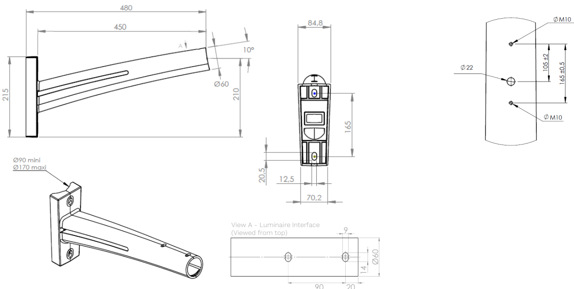
ELAYA WALL / LATERAL S480
